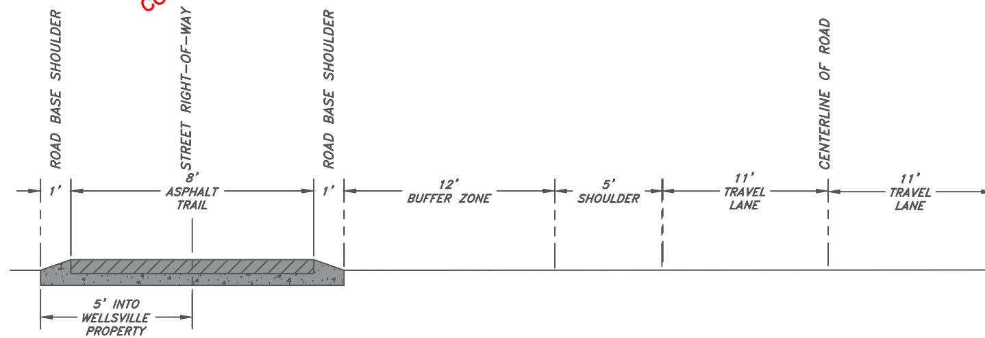
200 EAST CROSS SECTION ALONG CITY PROPERTY
