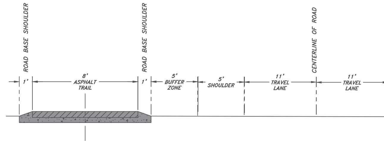
200 EAST CROSS SECTION NORTH OF 500 SOUTH
