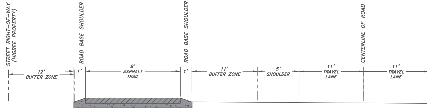
700 SOUTH CROSS SECTION ALONG HIGBEE PROPERTY
