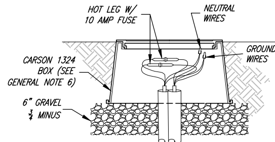
JUNCTION BOX WITH FUSES
