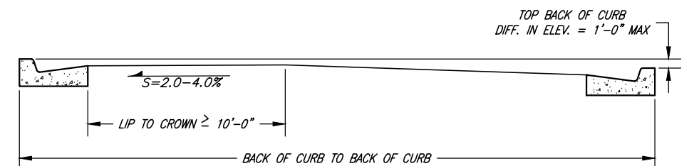
CROWN LOCATION FOR VARIOUS CROSS SLOPES
