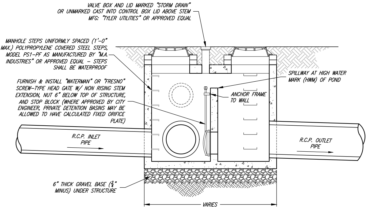
SECTION B-B
