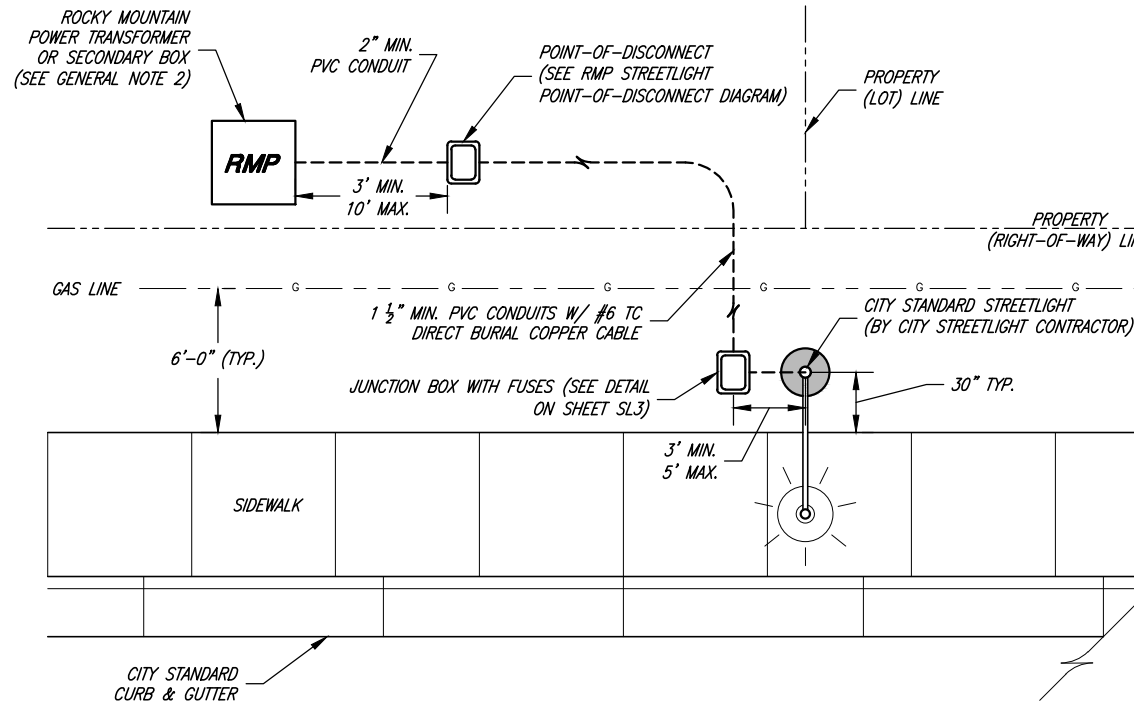
TYPICAL CONDUIT AND POWER LAYOUT "B" (STANDARD LOCAL STREET SECTION WITHOUT PARKSTRIP)
