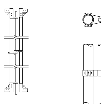
DROP ROD ASSEMBLY
