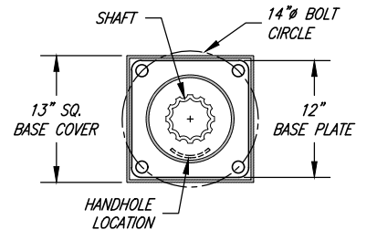
LP-1, LP-2, AND LP-3 BOLT PATTERN ANCHOR BOLT TEMPLATE NUMBER: TMP-89
